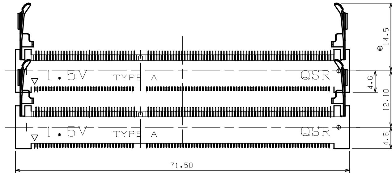
推奨基板レイアウト寸法 RECOMMENDED MOUNTAINING P.C. BOARD PATTERN LAYOUT DIM.
