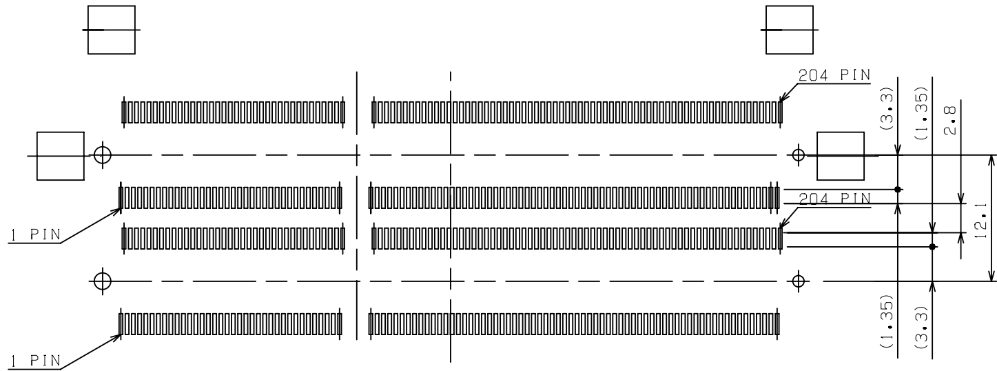
推奨基板レイアウト寸法 RECOMMENDED MOUNTAINING P.C. BOARD PATTERN LAYOUT DIM.
